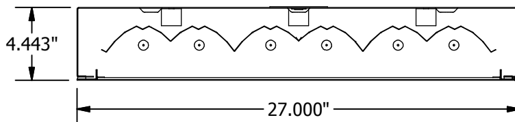
END VIEW
